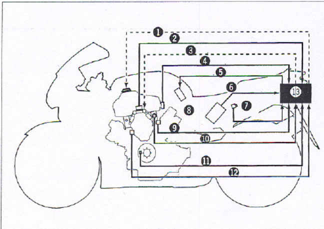
PGM-FI System
